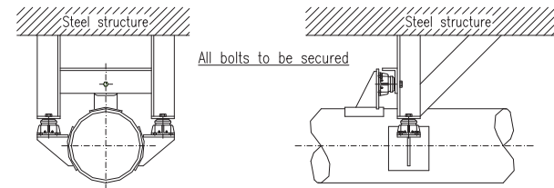
Horizontal pipe, example at 3 pcs.
