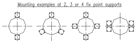
Fix point support at top penetration
