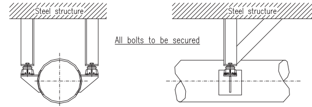
Horizontal pipe, example at 2 pcs.
